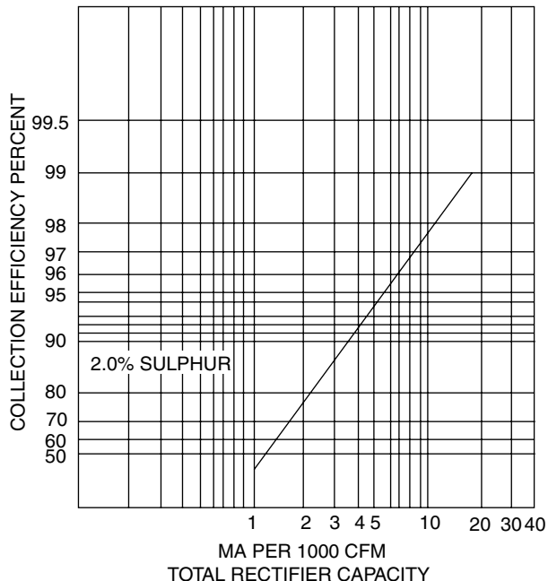
FIGURE 7 Precipitator design curve.
