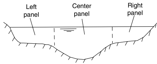
FIGURE 11 River channel division.
