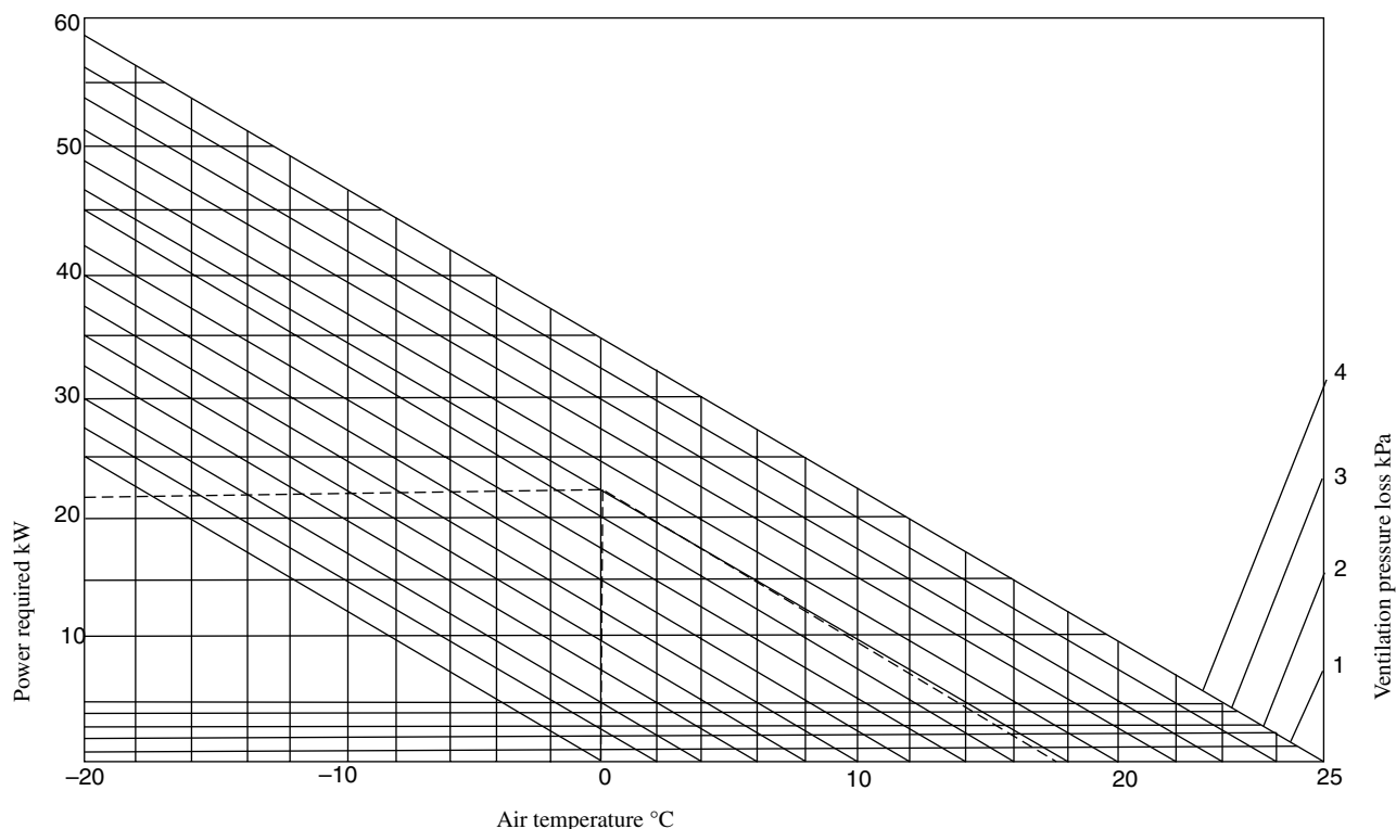
FIGURE 8 Chart for estimating energy requirements for heating.
