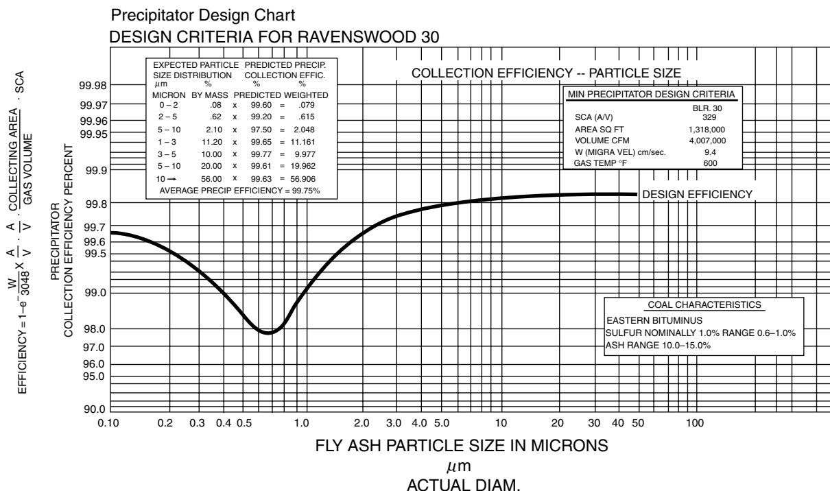
FIGURE 13 Precipitator collection efficiency as a function of particle size.
