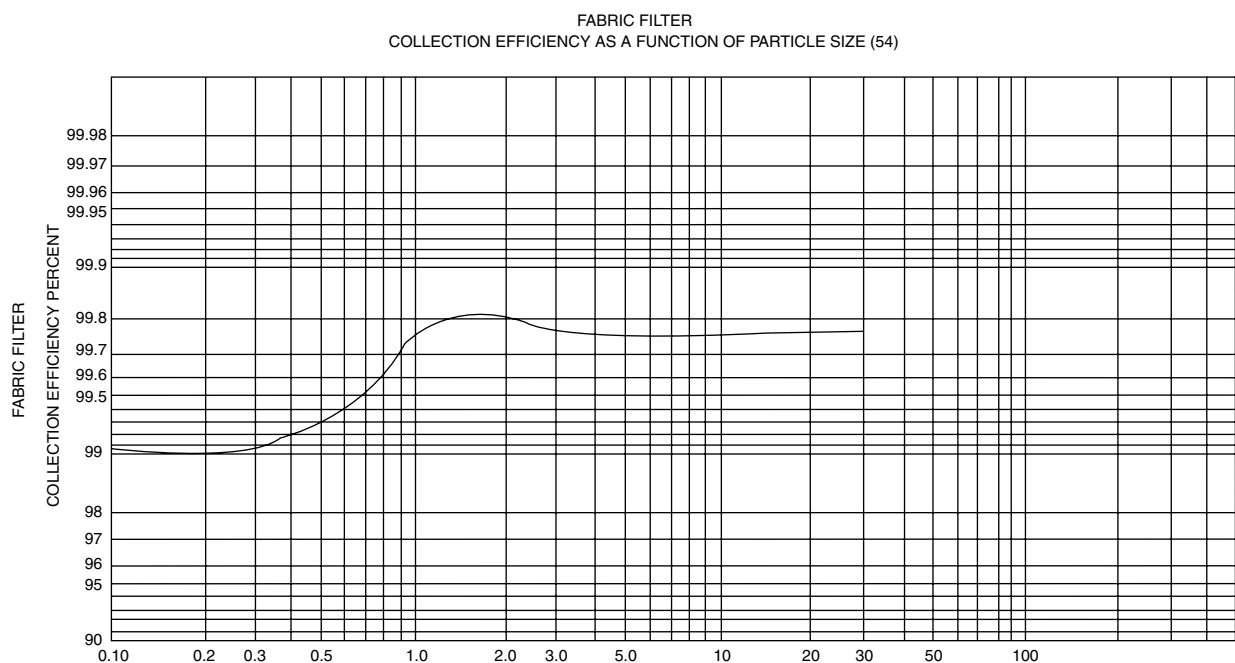
FIGURE 15 Fly ash particle size in microns, actual diameter.
