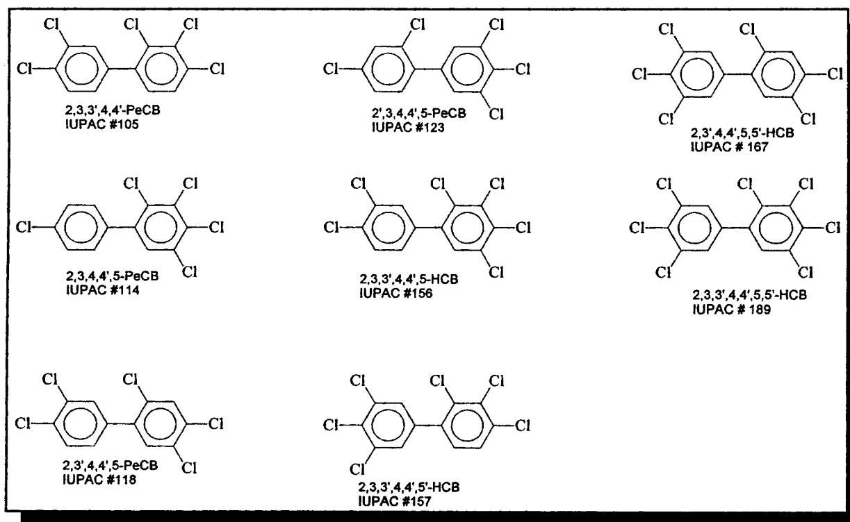
FIGURE 12 Mono-ortho-chlorobiphenyls.
