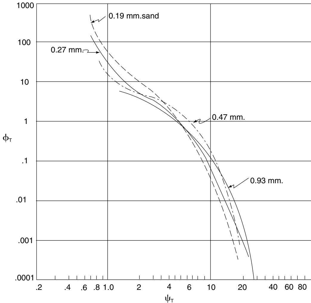
FIGURE 11 Bed material transport function (after Bishop et al. ).
