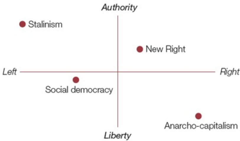
Figure 1.5 Two-dimensional spectrum
