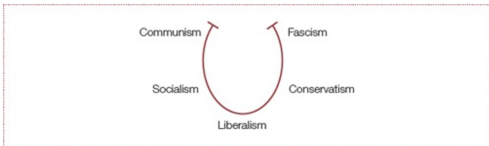
Figure 1.4 Horseshoe spectrum
