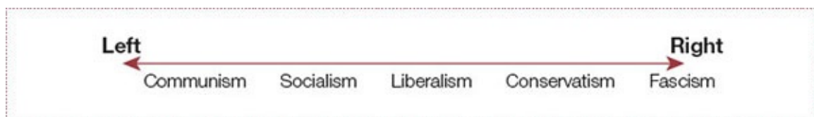
Figure 1.3 Linear spectrum
